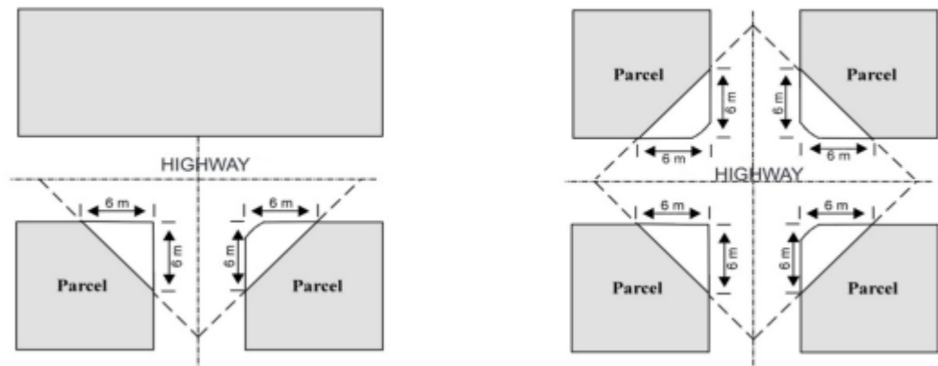
SIGHT TRIANGLE
