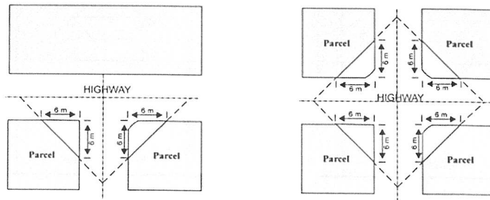
SIGHT TRIANGLE
